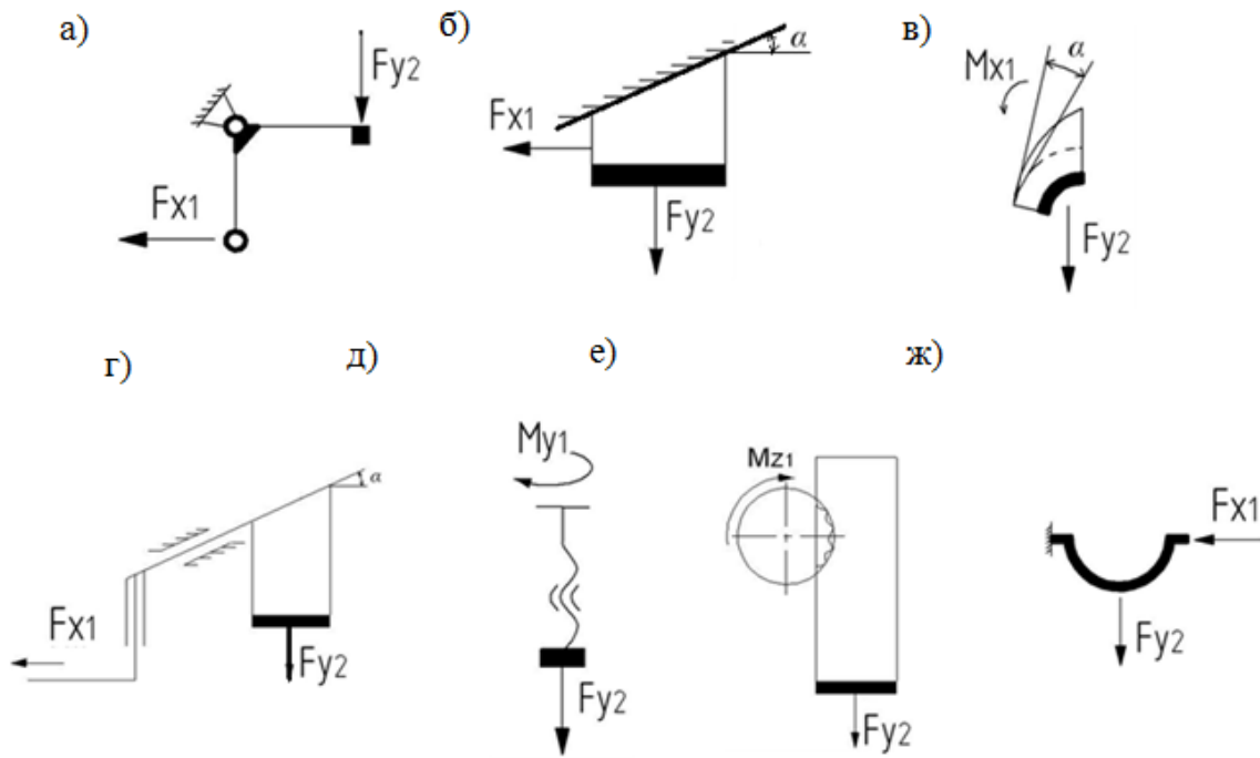
Fig. 4. Solid-state simplest mechanical transducers of displacement and forces: a - lever (LV); b - wedge (WD); c - spiral (SP); d - plunger (PL); e - screw (SC); f - gear (GR); g - spring (SR)
